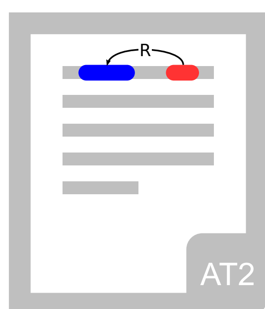
Relation annotation
