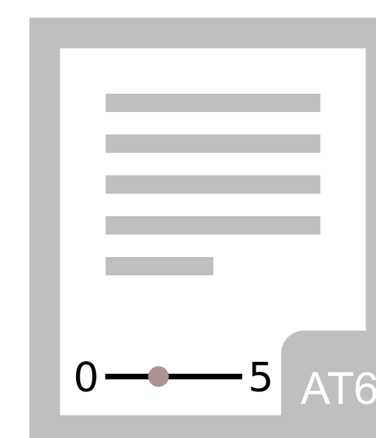
Numerical annotation
