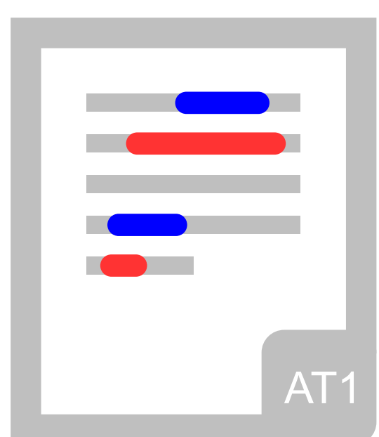
Span labeling
