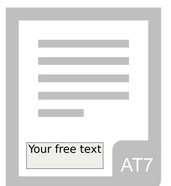
Free-text annotation
