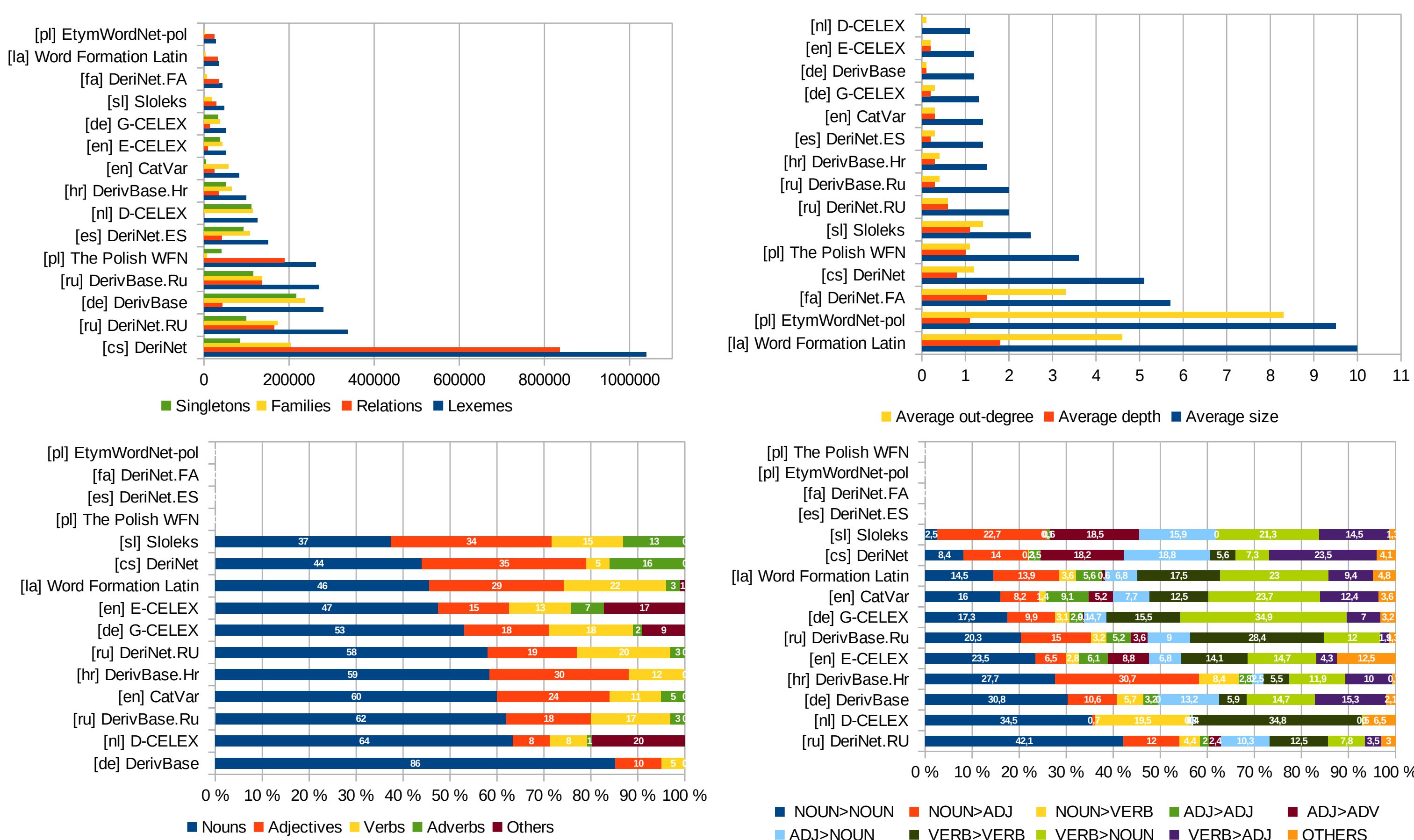
Figure: Quantitative comparison between DeriNet.RU and the 15 largest resources from the Universal Derivations collection.
